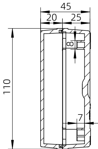
长侧边 (Side section)
