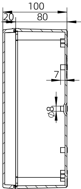
长侧边 (Side section)
